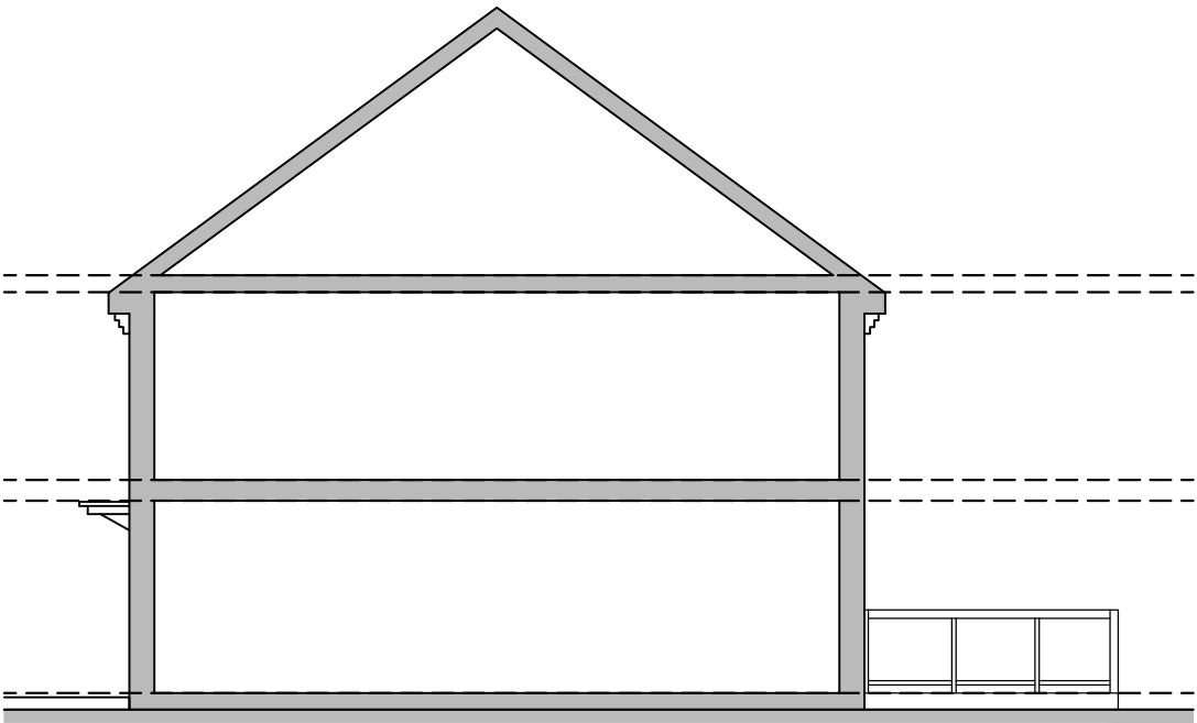
SECTION 1:100
