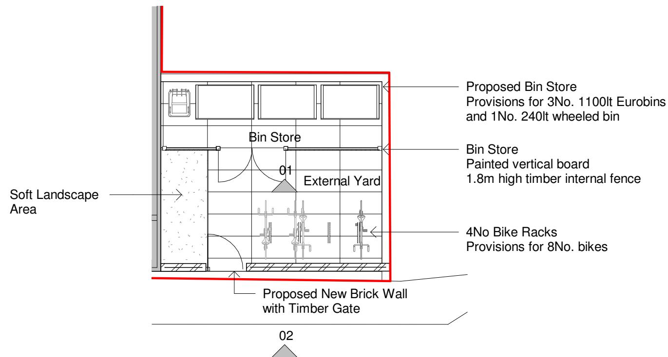
1 Bin Store Plan 1 : 100
