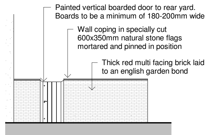
3 Proposed Fence Elevation - 02 1 : 100
