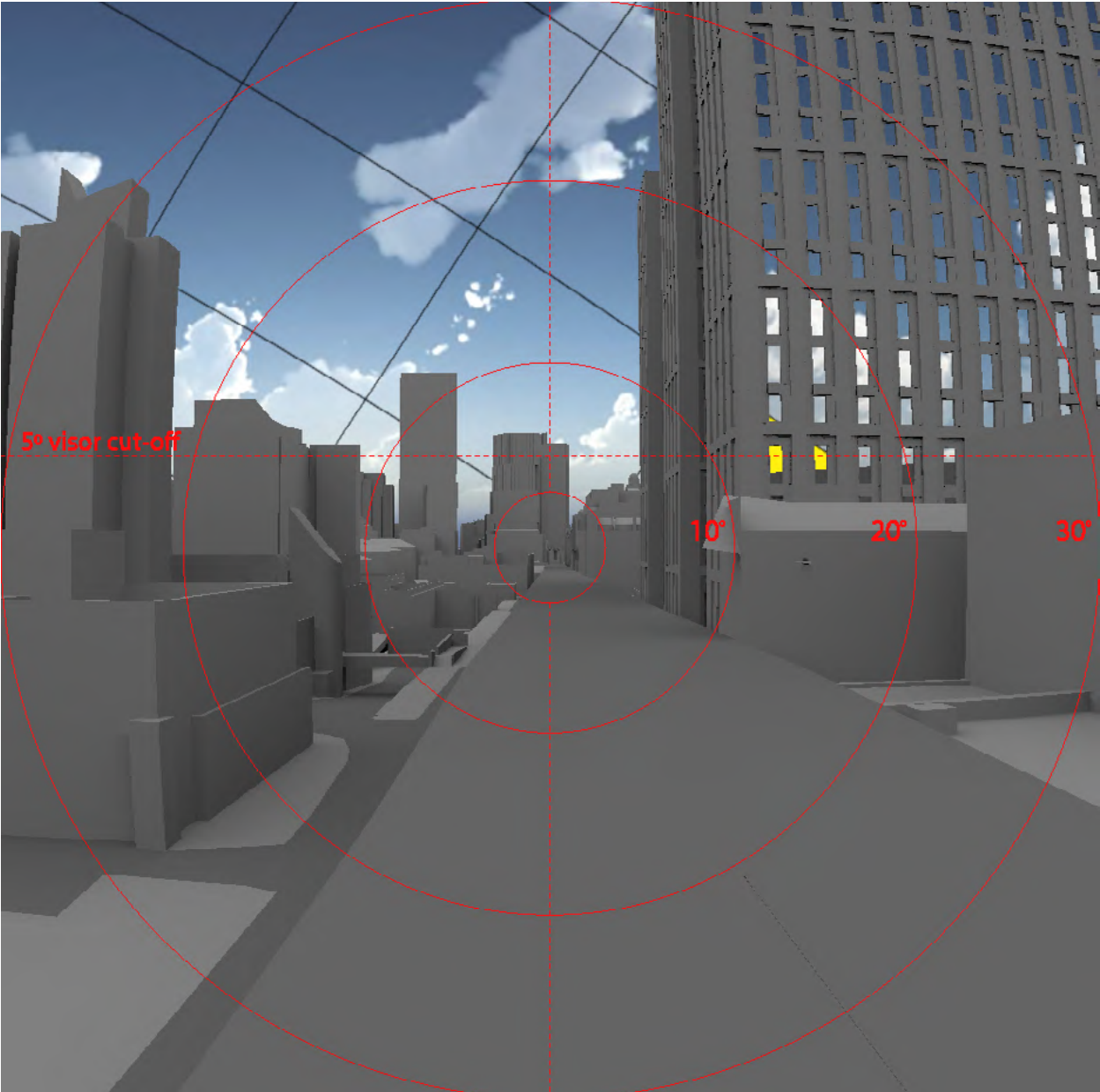
Fig. 23: Solar reflections
