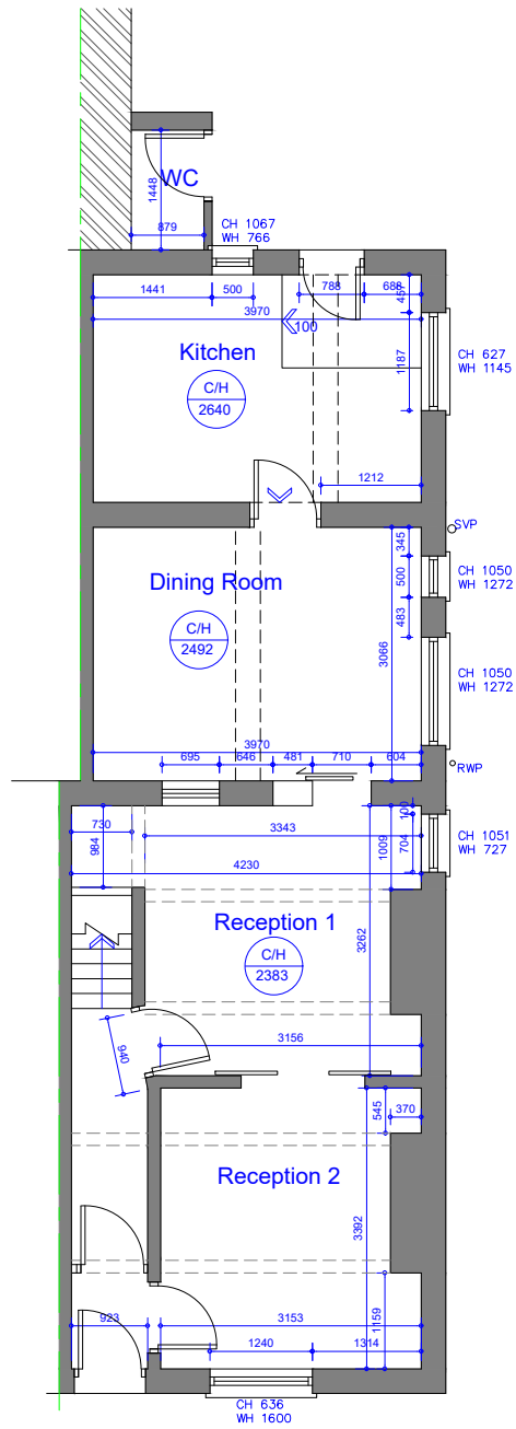
Existing Ground Floor Plan Scale 1:100
