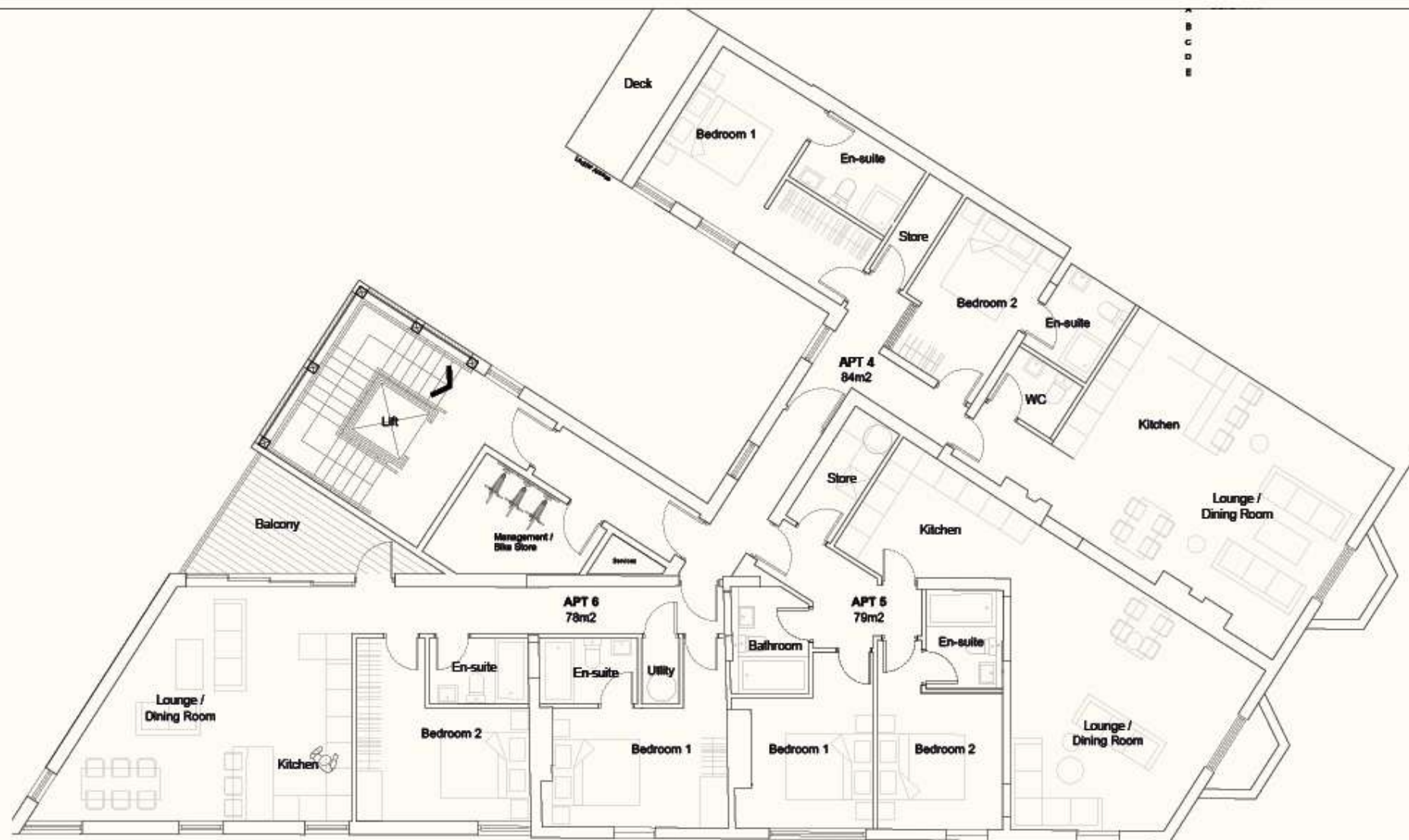
⌚ PROPOSED SECOND FLOOR
