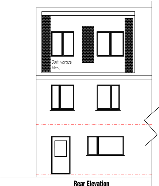
Rear Elevation
