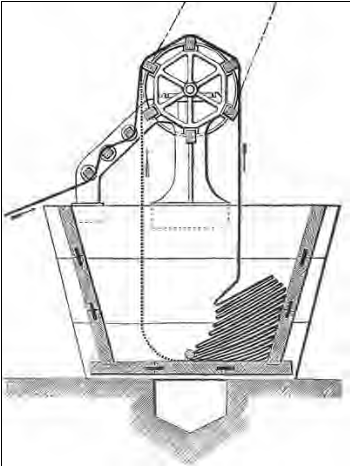
Plate 199: Diagram of a wince dye beck or dye digger
