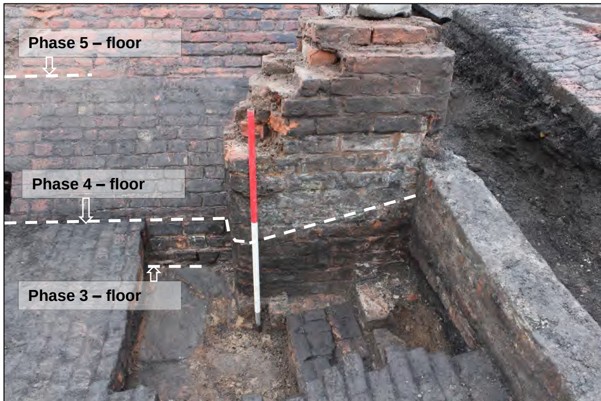
Plate 131: The three successive charging floors revealed within the southern half of the boiler house: 3172 (Phase 3); 3065 (Phase 4) and 3174 (Phase 5). Photographed looking south (1m scale)
