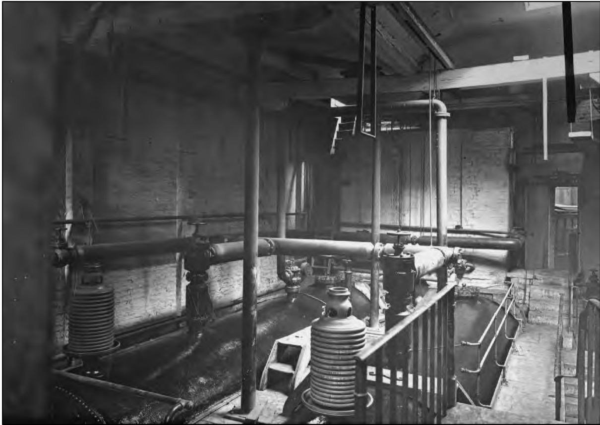
Plate 189: Photograph showing the two steam boilers at Mayfield Baths
