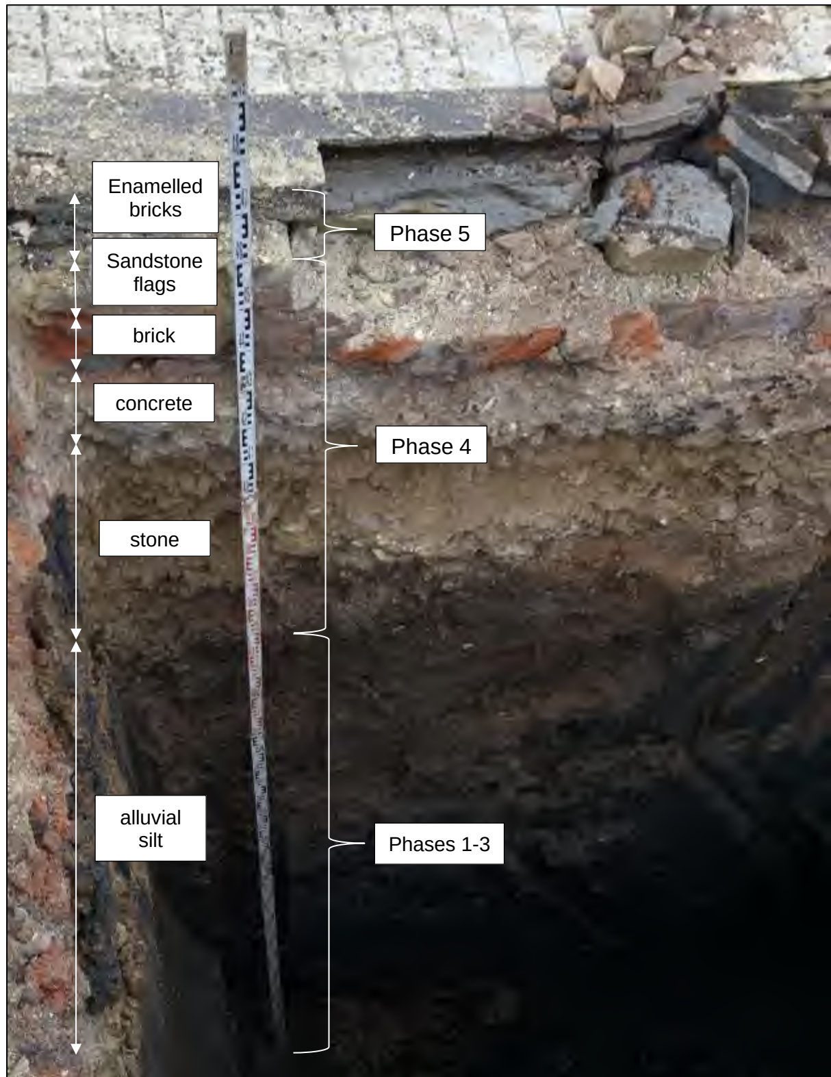
Plate 49: Sondage through the base of Pool 226 showing the composition of the foundations above earlier layers of alluvial silt
