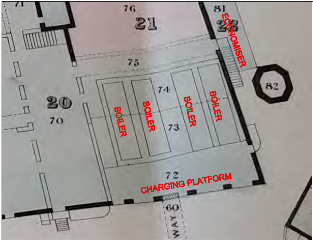
Plate 201: Extract from the 1872 insurance plan showing the internal layout of the boiler house
