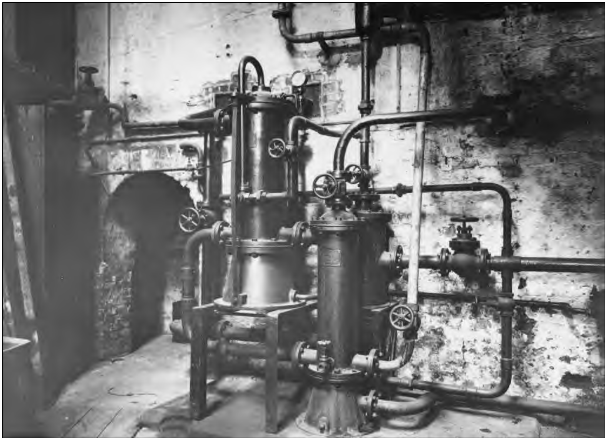
Plate 14: The Royle Calorifier at Mayfield Baths, 1902.
