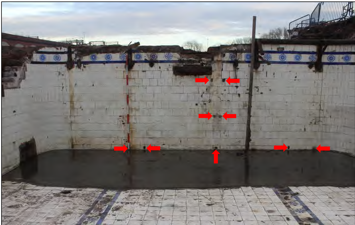
Plate 62: The eastern end of Pool 225 showing the position of the fixings for the steam injection pipe (removed) and L-shaped brackets visible above the waterline (2m scale)
