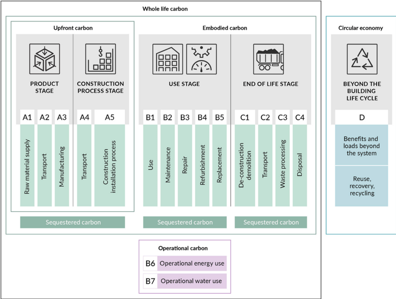
Figure 4 System Boundary: EN 15978:2011 Display of modular information for the different stages of the building assessment
