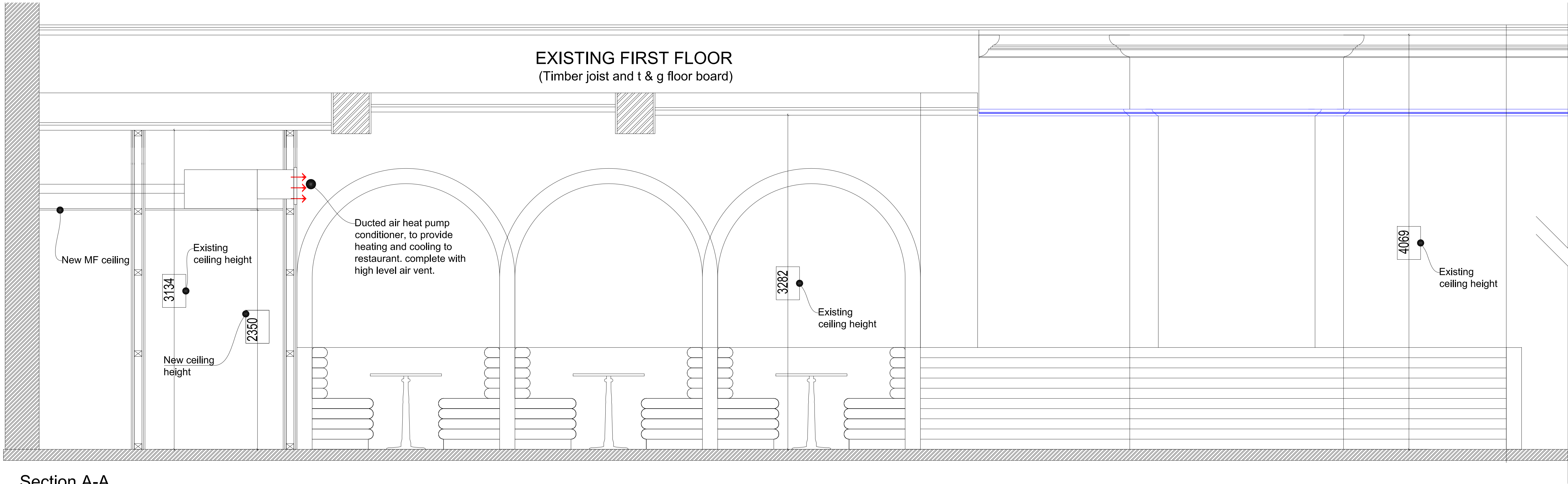
Section A-A Ground Floor scale A1@1:20
