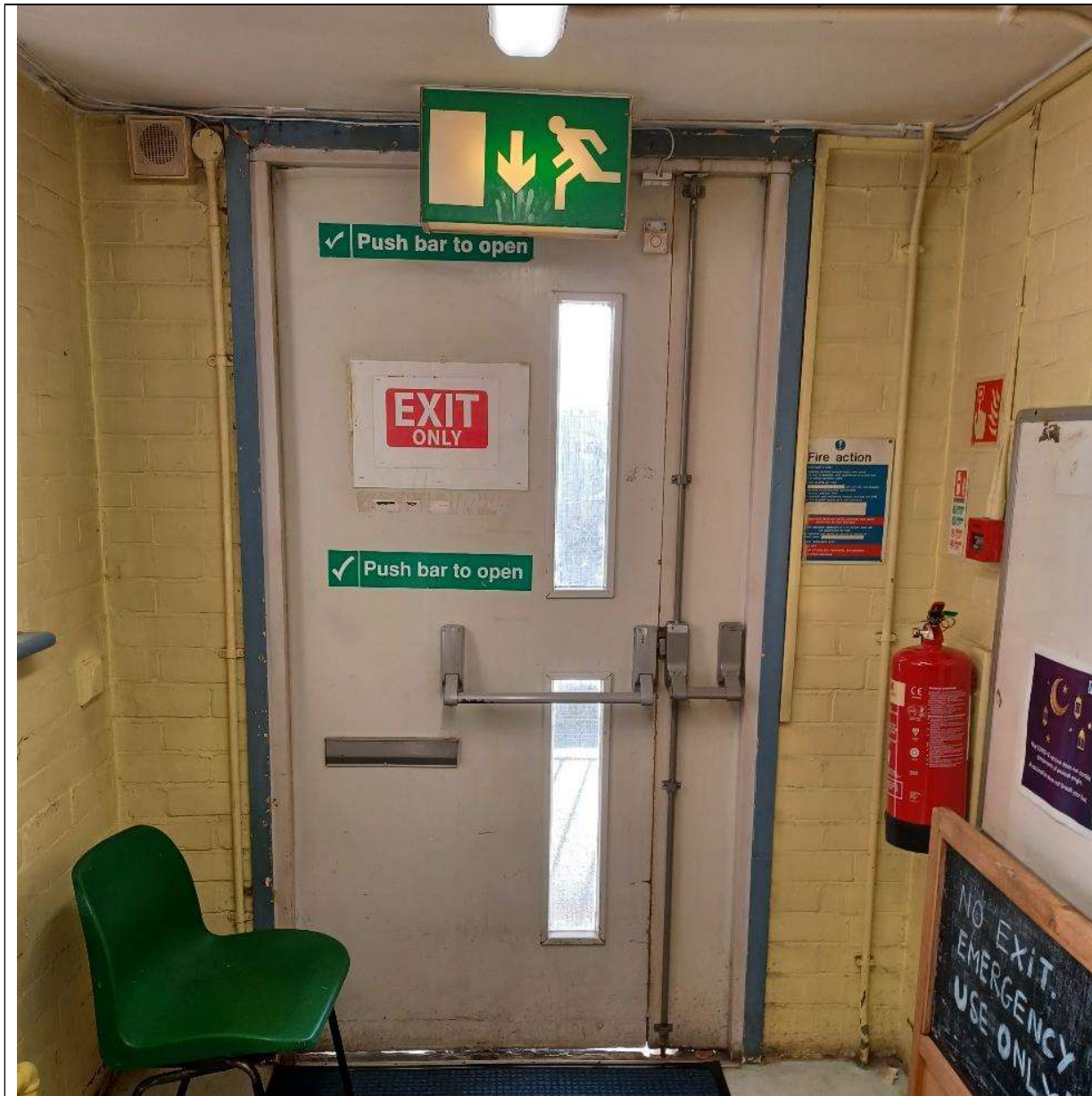
Photograph: 2 - Ceiling mounted exit sign – does not comply with BS 5499
