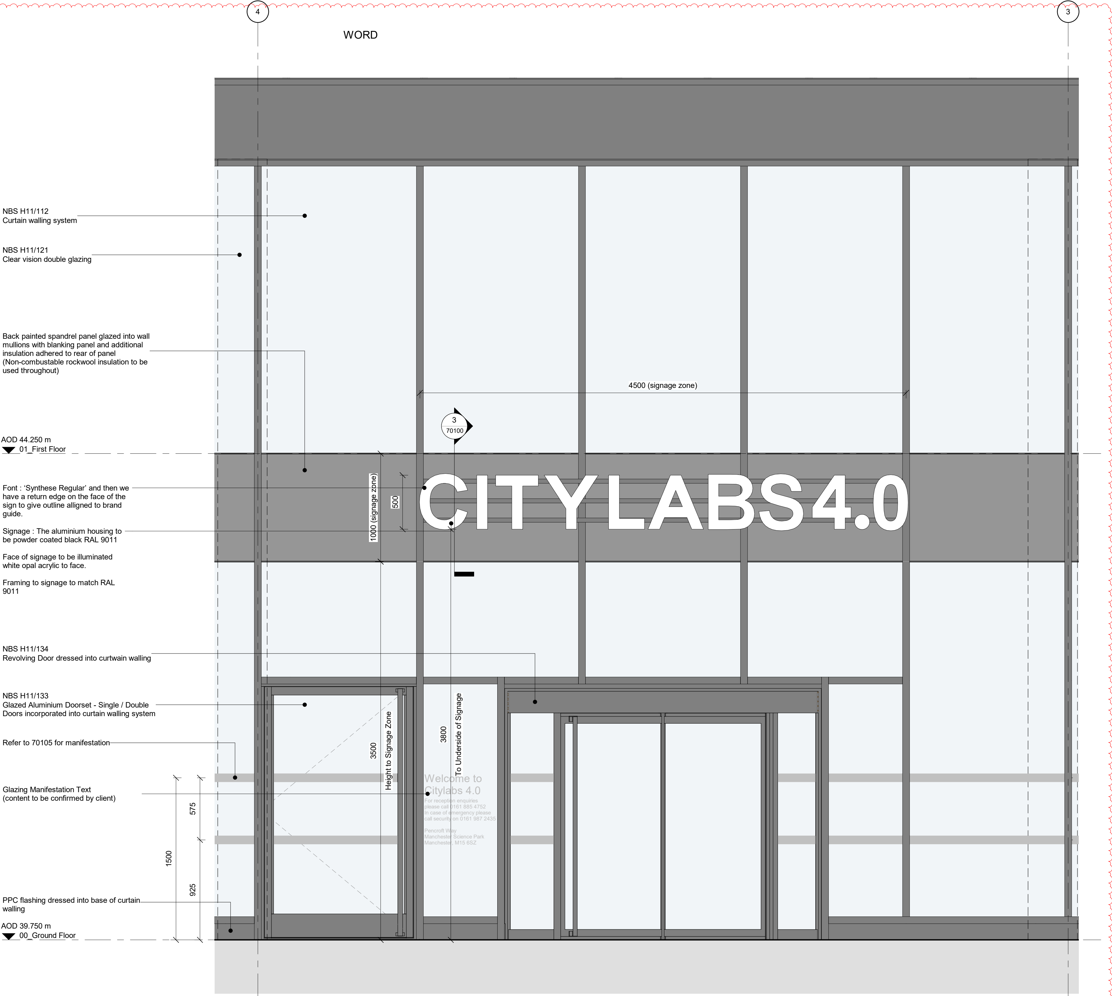
External Signage (Low Level) and Manifestation 1 : 20
