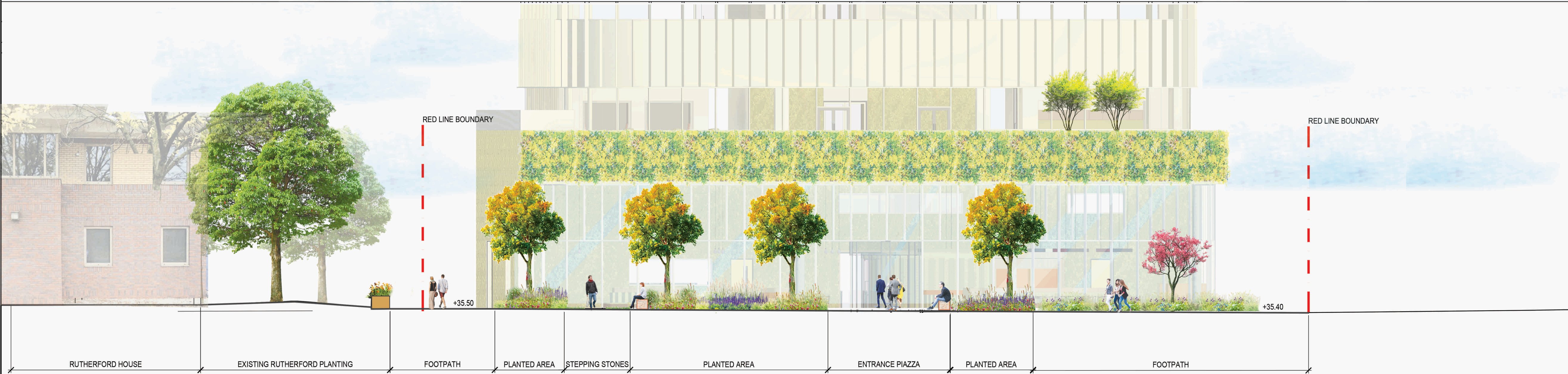
SECTION D-D' SCALE 1:100
