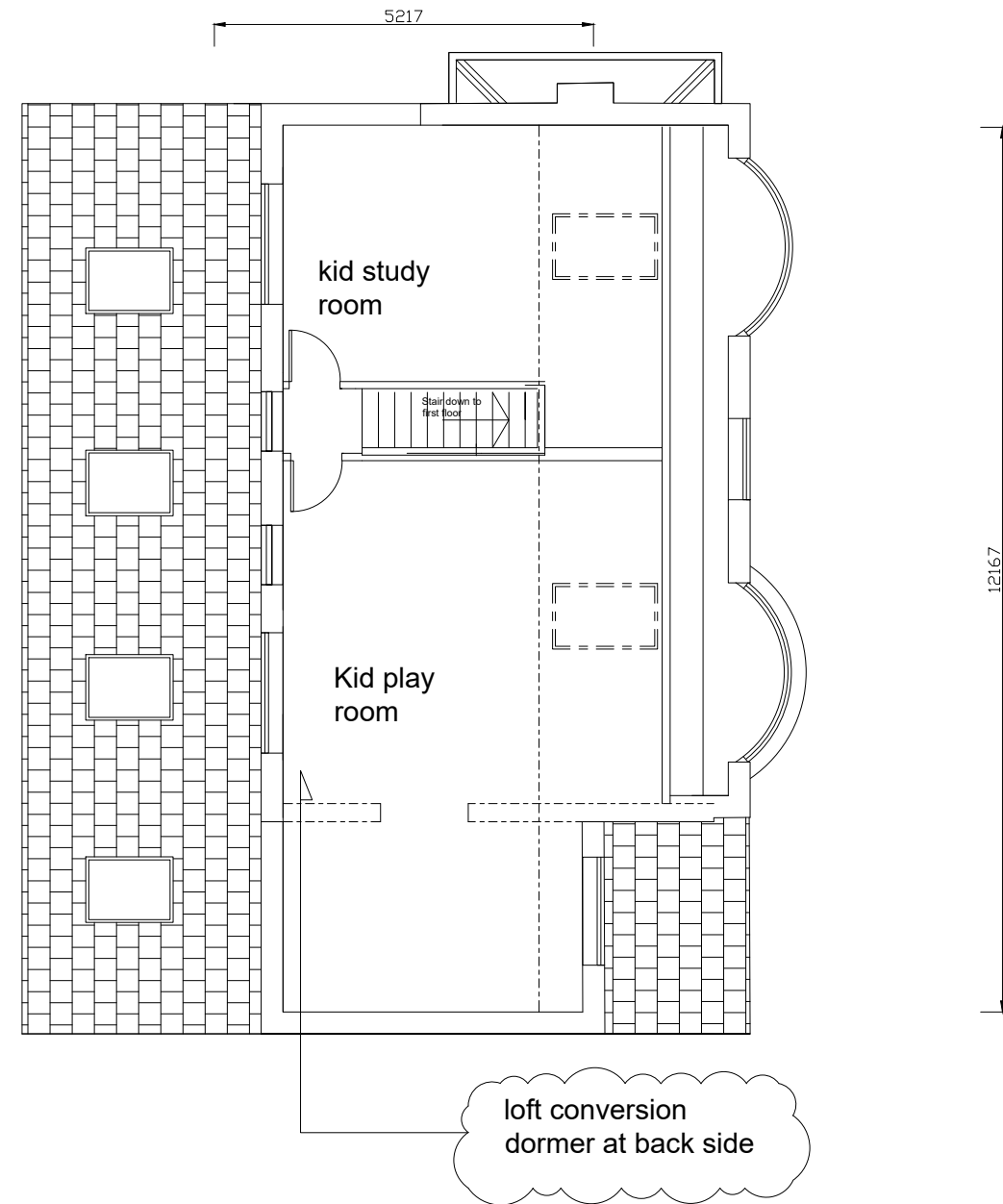
- LAYOUT FLOOR PLAN PROPOSED PLAN Loft 1 : 100 ( IN A3)
