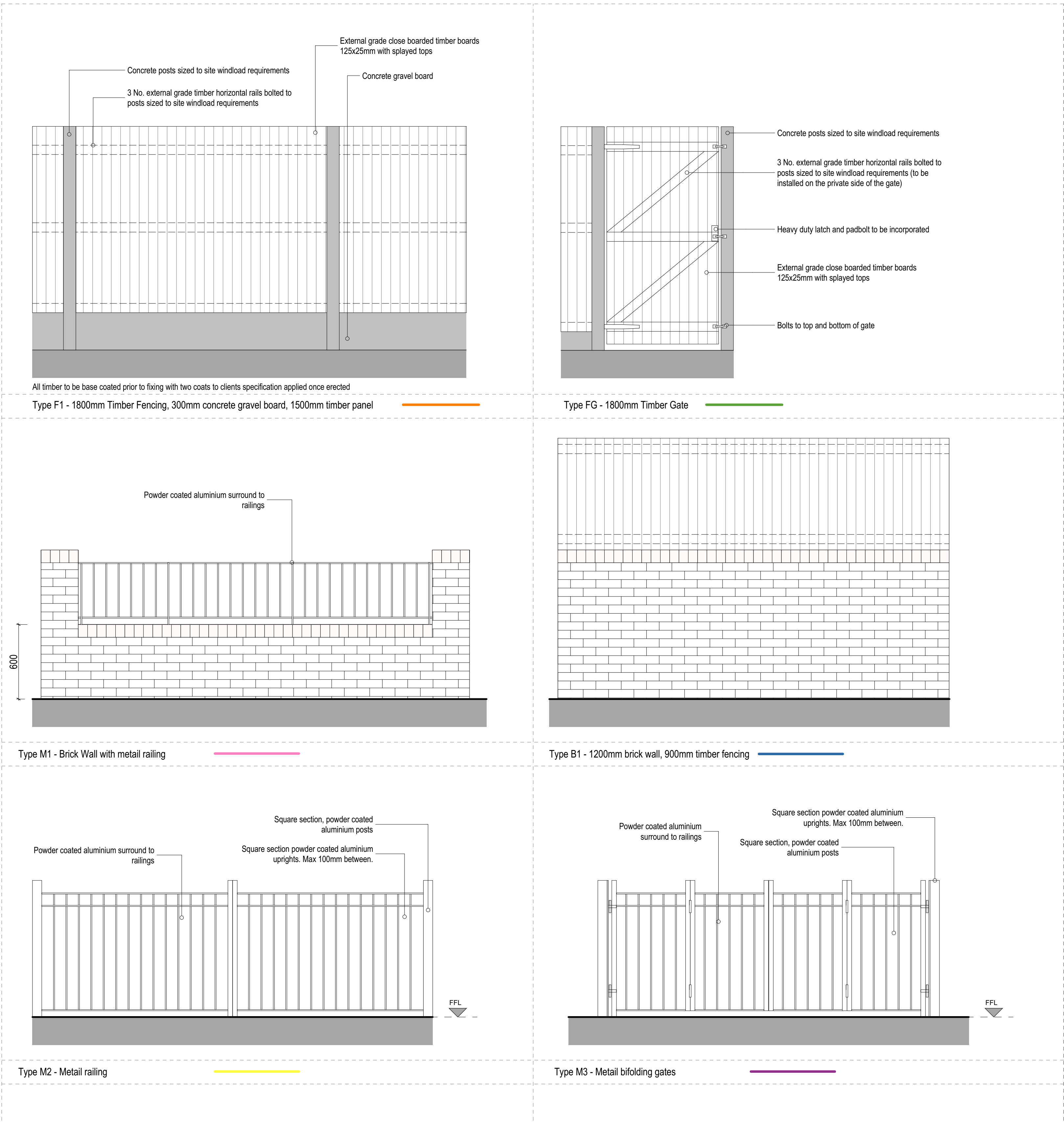
1 Boundary Details 1:20
