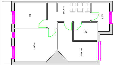
EXISTING FIRST FLOOR PLAN SCALE - 1:100@A1
