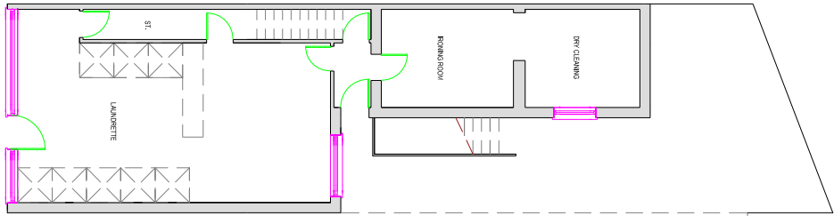
EXISTING GROUND FLOOR PLAN SCALE - 1:100@A1
