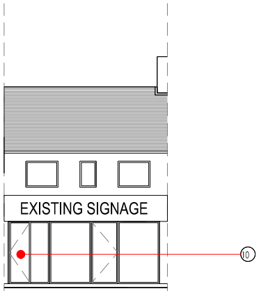
PROPOSED FRONT ELEVATION SCALE - 1:100@A1
