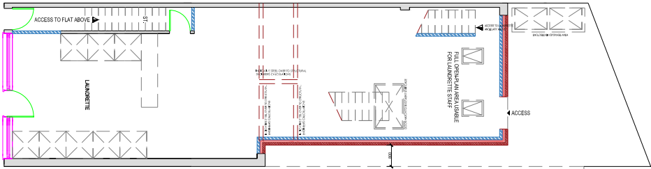
PROPOSED GROUND FLOOR PLAN SCALE - 1:100@A1
