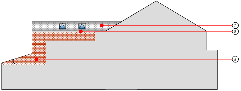
PROPOSED SIDE ELEVATION SCALE - 1:100@A1
