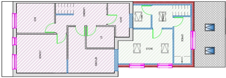
PROPOSED FIRST FLOOR PLAN SCALE - 1:100@A1
