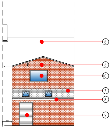
PROPOSED REAR ELEVATION SCALE - 1:100@A1
