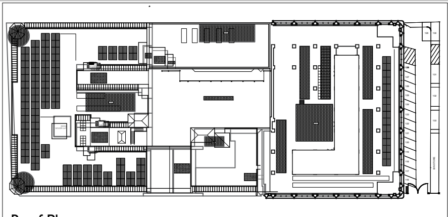
Roof Plan Scale 1:500
