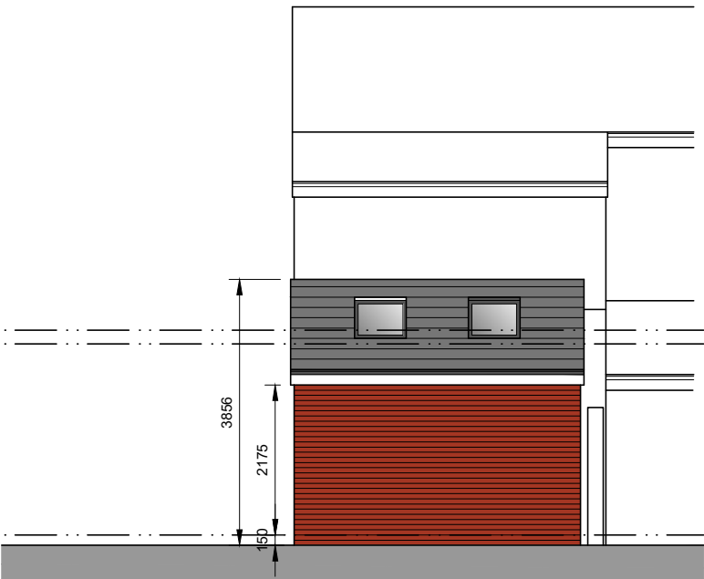
South Facing Rear Elevation
