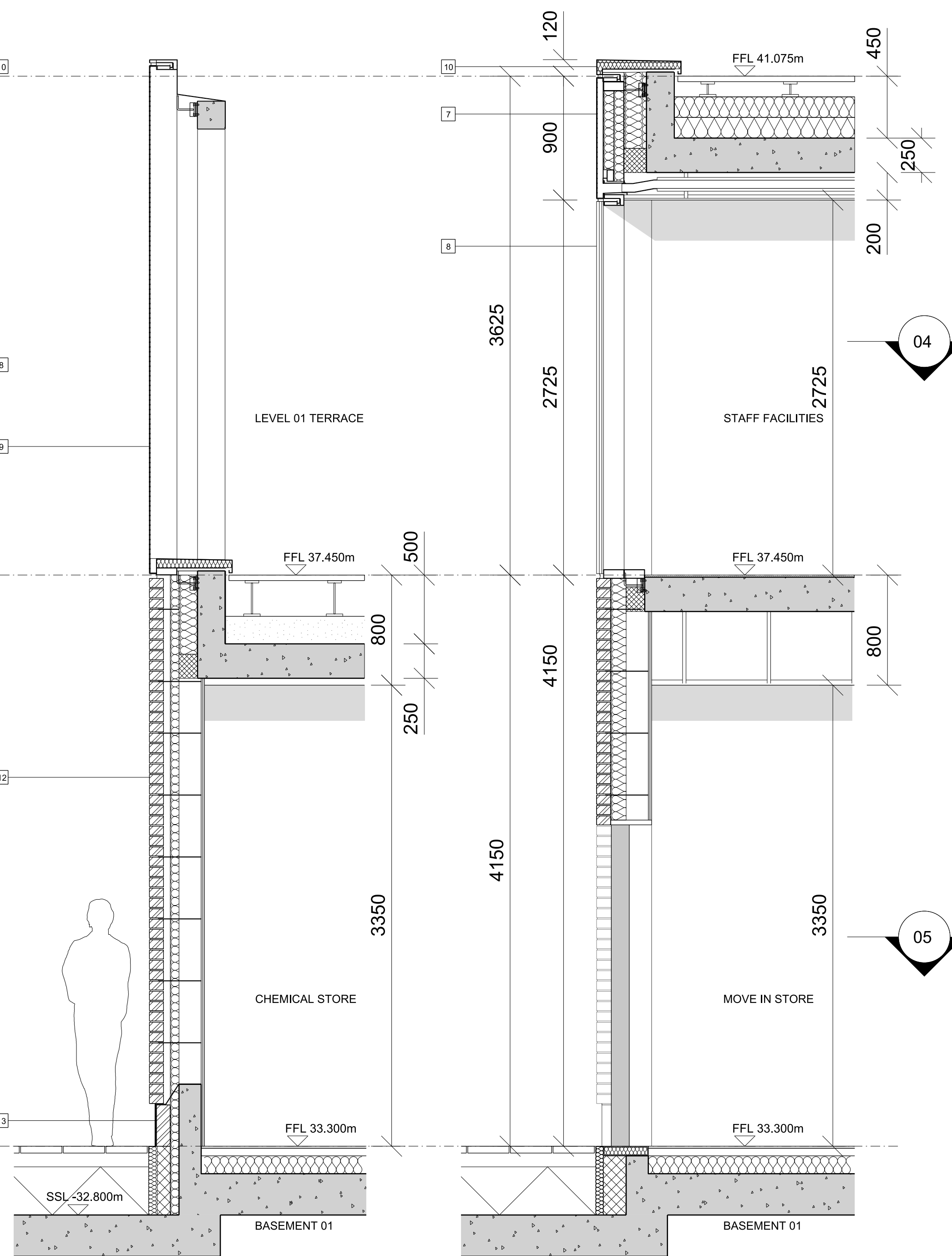
02 Podium Facade Detail Detail Section
