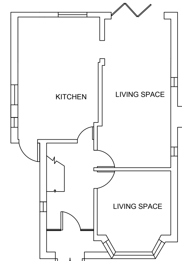
PROPOSED - ground
