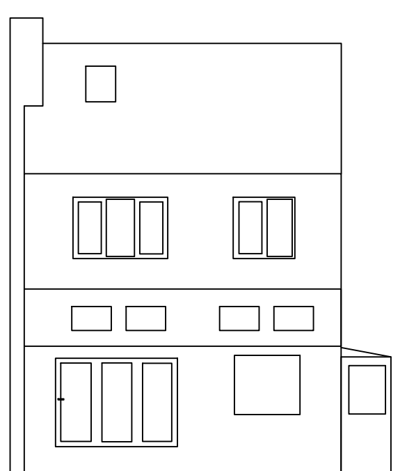
EXISTING - rear
