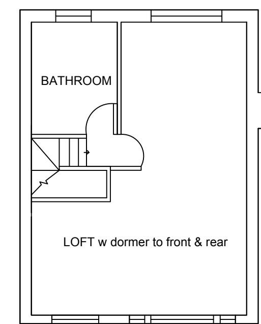
PROPOSED - loft
