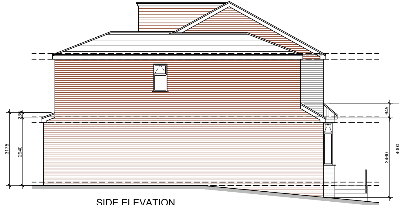
SIDE ELEVATION 1:100
