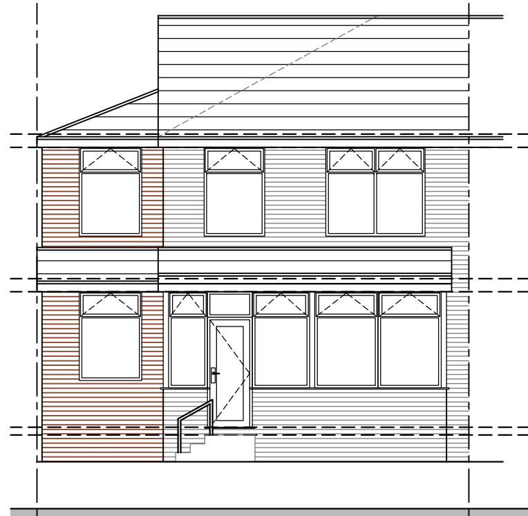
FRONT ELEVATION 1:100
