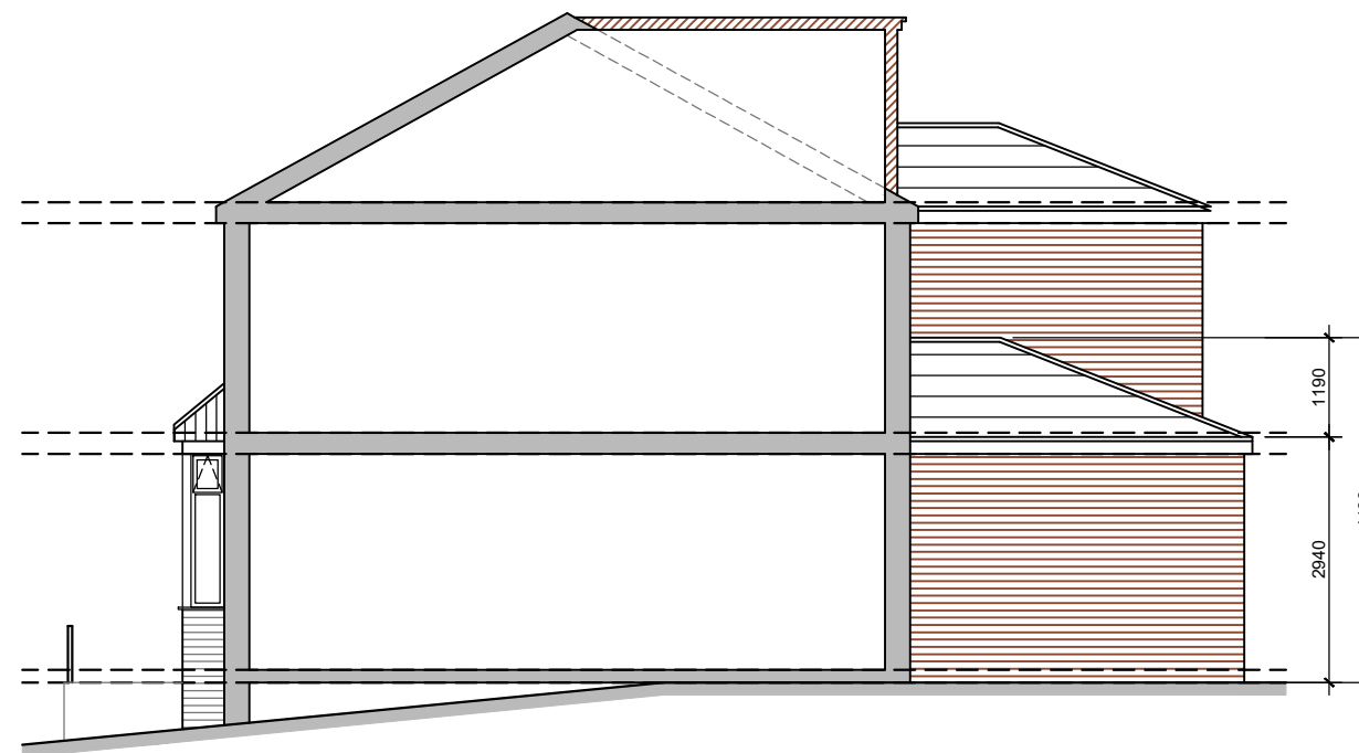
SIDE ELEVATION 1:100
