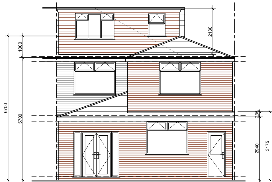
REAR ELEVATION 1:100
