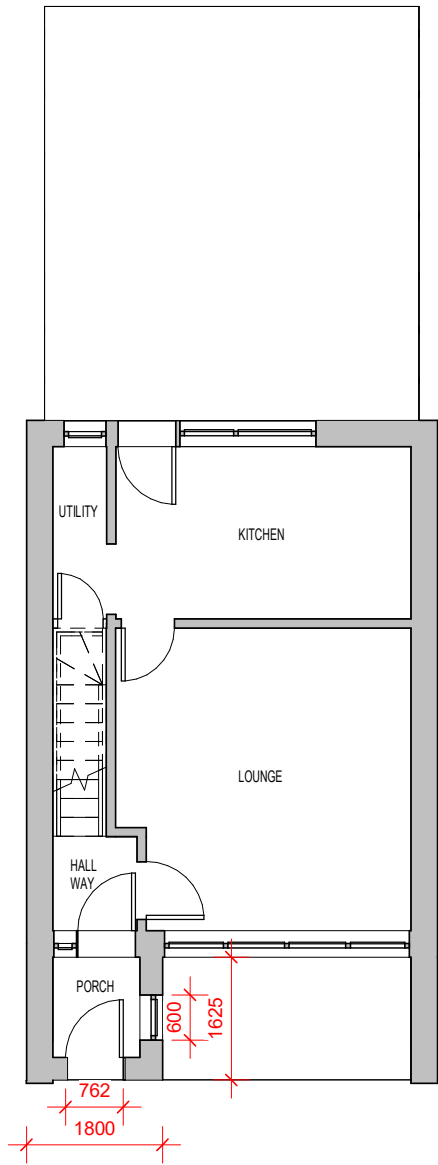
1 Ground Floor 1 : 100
