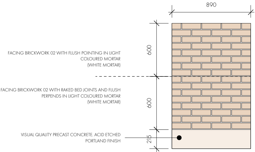
INITIAL SAMPLE PANEL TO BE CONSTRUCTED TO ESTABLISH MORTAR COLOUR AND POINTING 1:25
