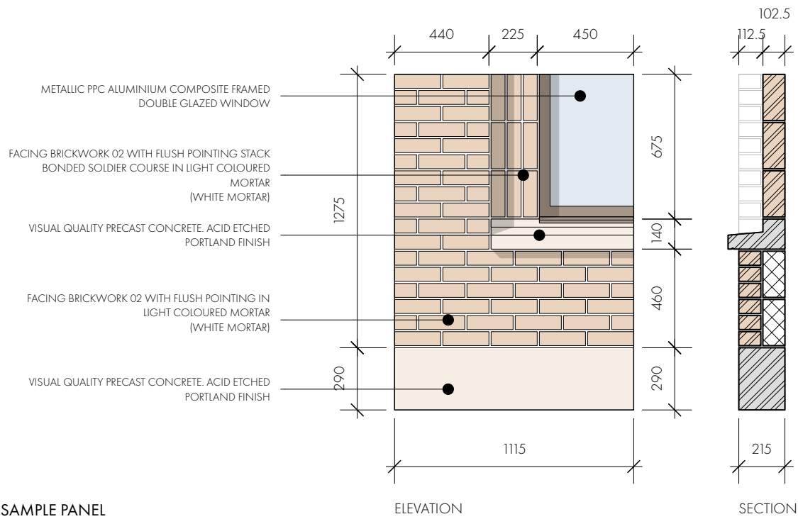
SAMPLE PANEL DEMONSTRATING KEY JUNCTIONS 1:25
