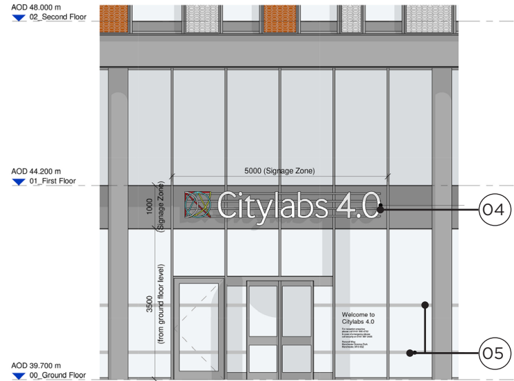
Type 02 - External Signage / Manifestation
