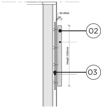
Type 01 - External Signage Section
