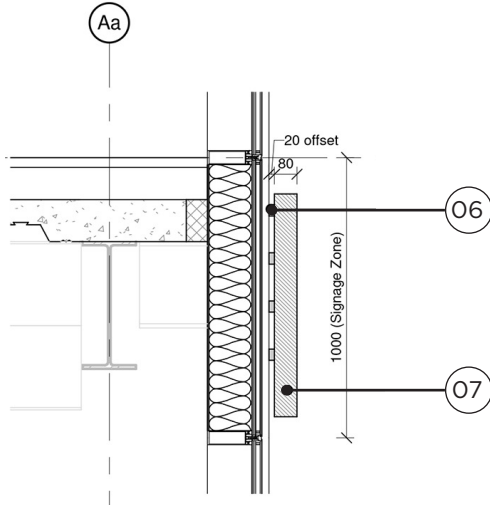
Type 02 - External Signage Section
