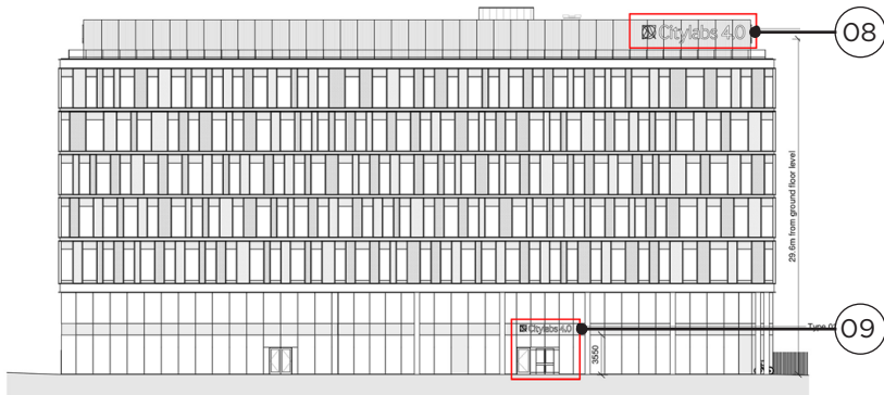
Signage / Manifestation on North Elevation
