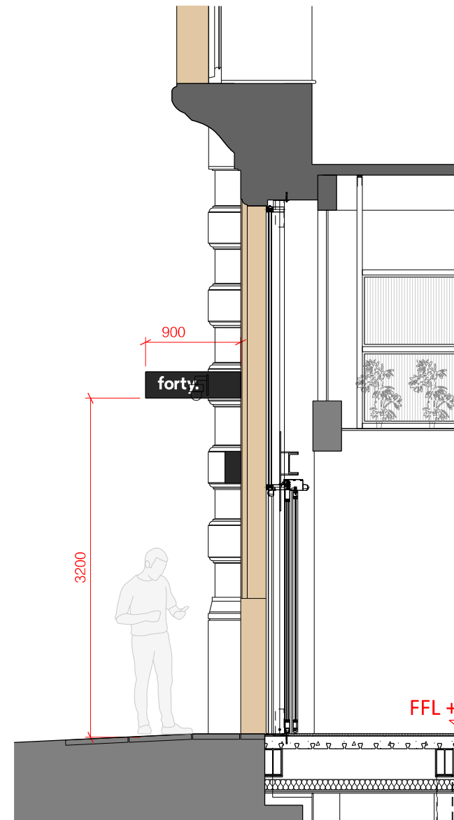
Proposed Section - Princess Street 1:50
