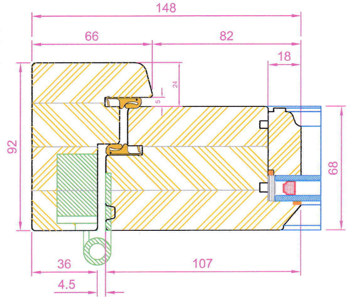
Section B-B
