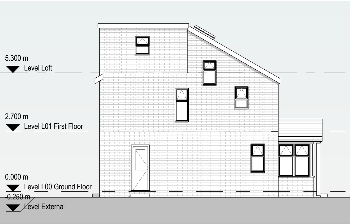
4 Existing East Elevation 1 : 100
