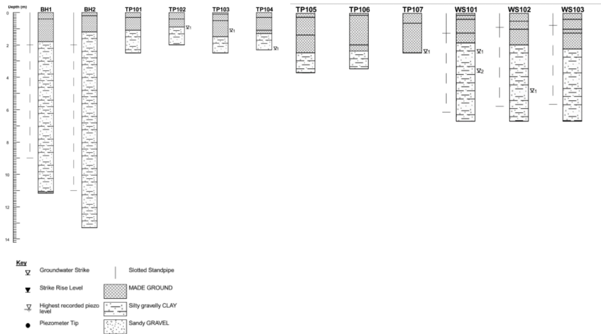
Plate 4-1: Summary of ground conditions.
