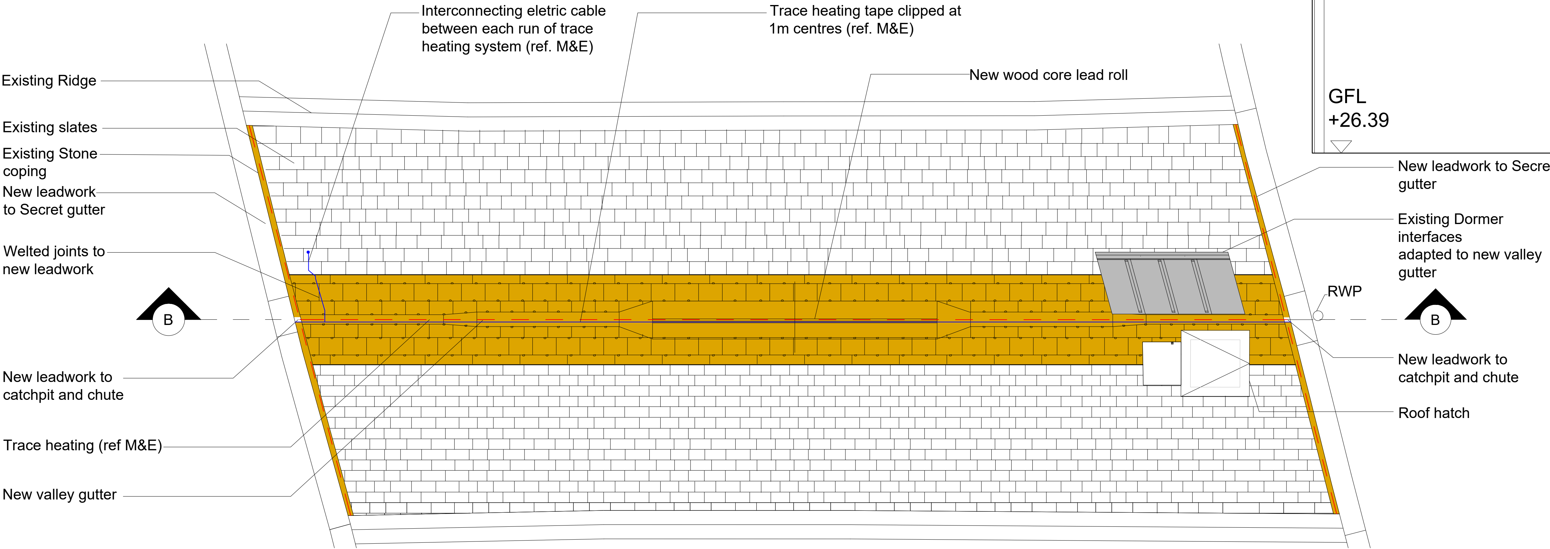
VALLEY GUTTER: PROPOSED WORKS TO BAY 02 GA SECTIONAL ELEVATION + PLAN 1:400 @ A3 1:200 @ A1
