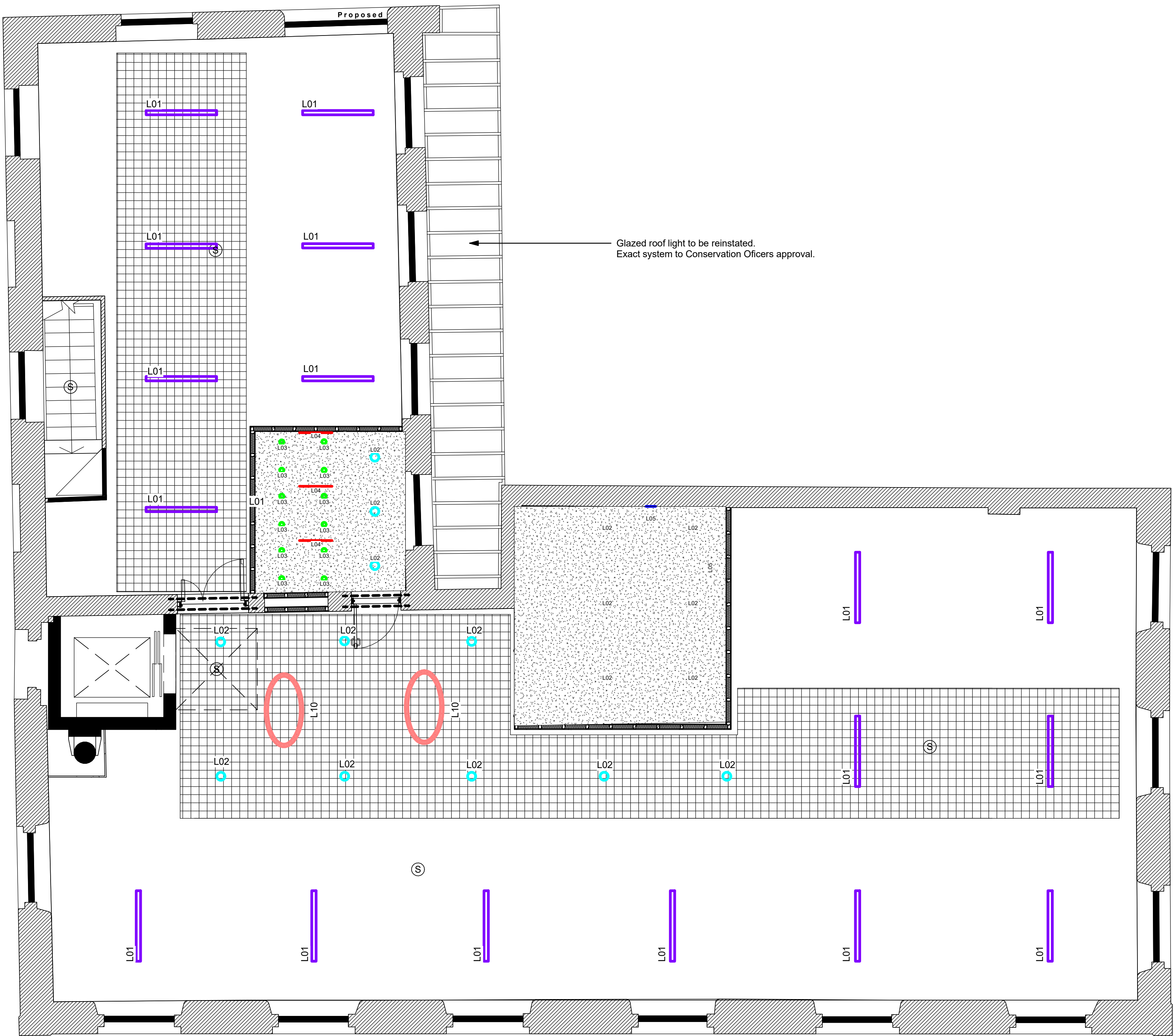
4FL Proposed Reflected Ceiling Layout Option 1
