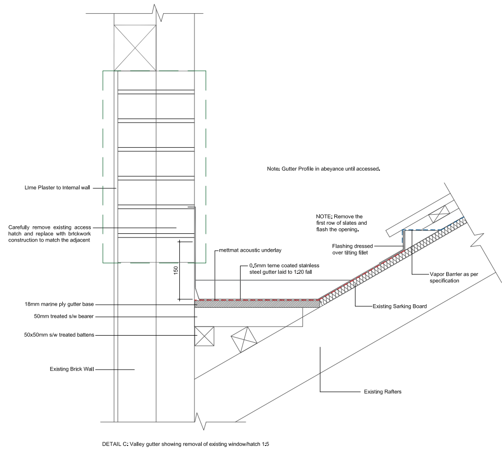
DETAIL C: Valley gutter showing removal of existing window/hatch 1:5
