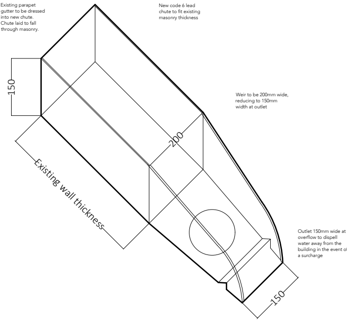
Rainwater Chute - Axonometric 1:10
