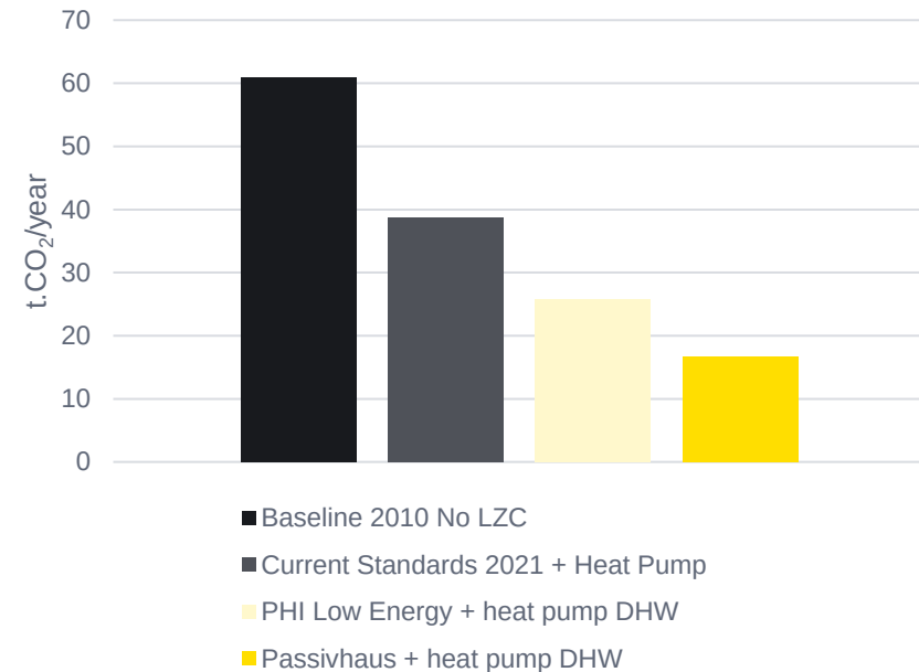
Figure 4: Energy efficiency and low carbon heat scenarios site CO 2 (See Appendix A for assumptions)
