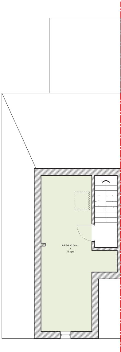
PROPOSED LOFT FLOOR PLAN 1:100 @ A3
