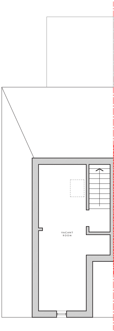
EXISTING LOFT FLOOR PLAN 1:100 @ A3
