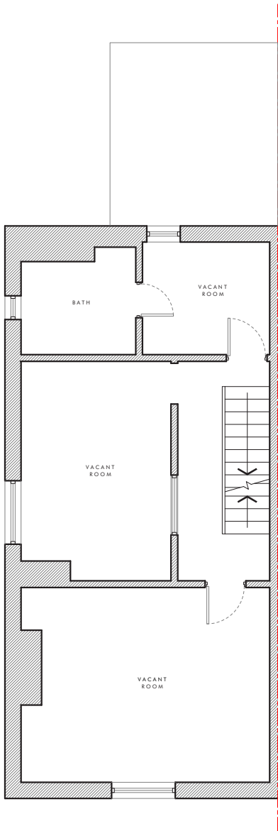
EXISTING FIRST FLOOR PLAN 1:100 @ A3
