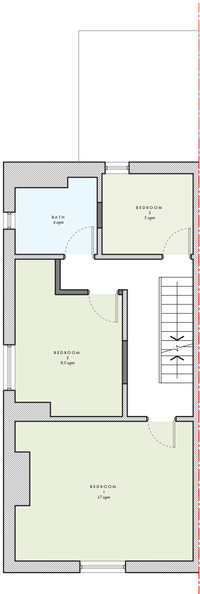
PROPOSED FIRST FLOOR PLAN 1:100 @ A3
