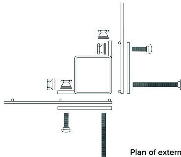
Plan of external corner
