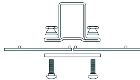
Plan of panels in line
