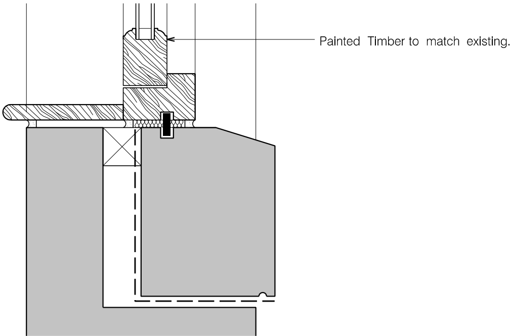
Section A – Typical Sill Detail Scale 1:5
