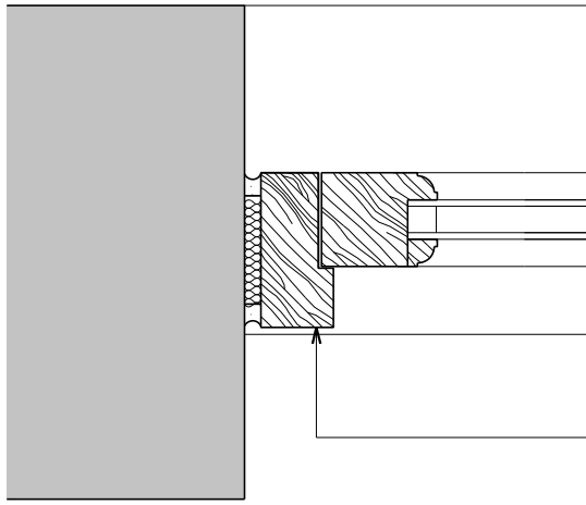
Section B – Typical Jamb Detail Scale 1:5
