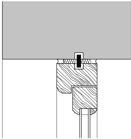
Section A – Typical Head Detail Scale 1:5
