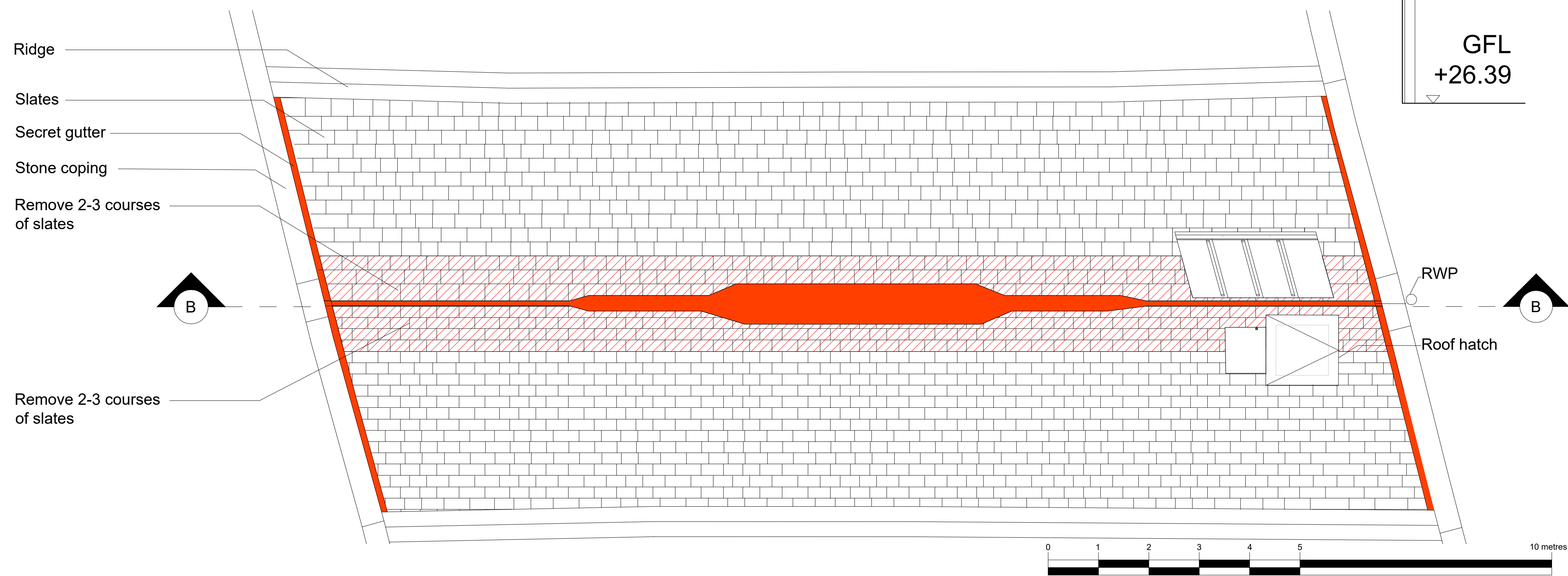
VALLEY GUTTER: EXISTING: BAY 02 GA SECTIONAL ELEVATION + PLAN 1:400 @ A3 1:200 @ A1
