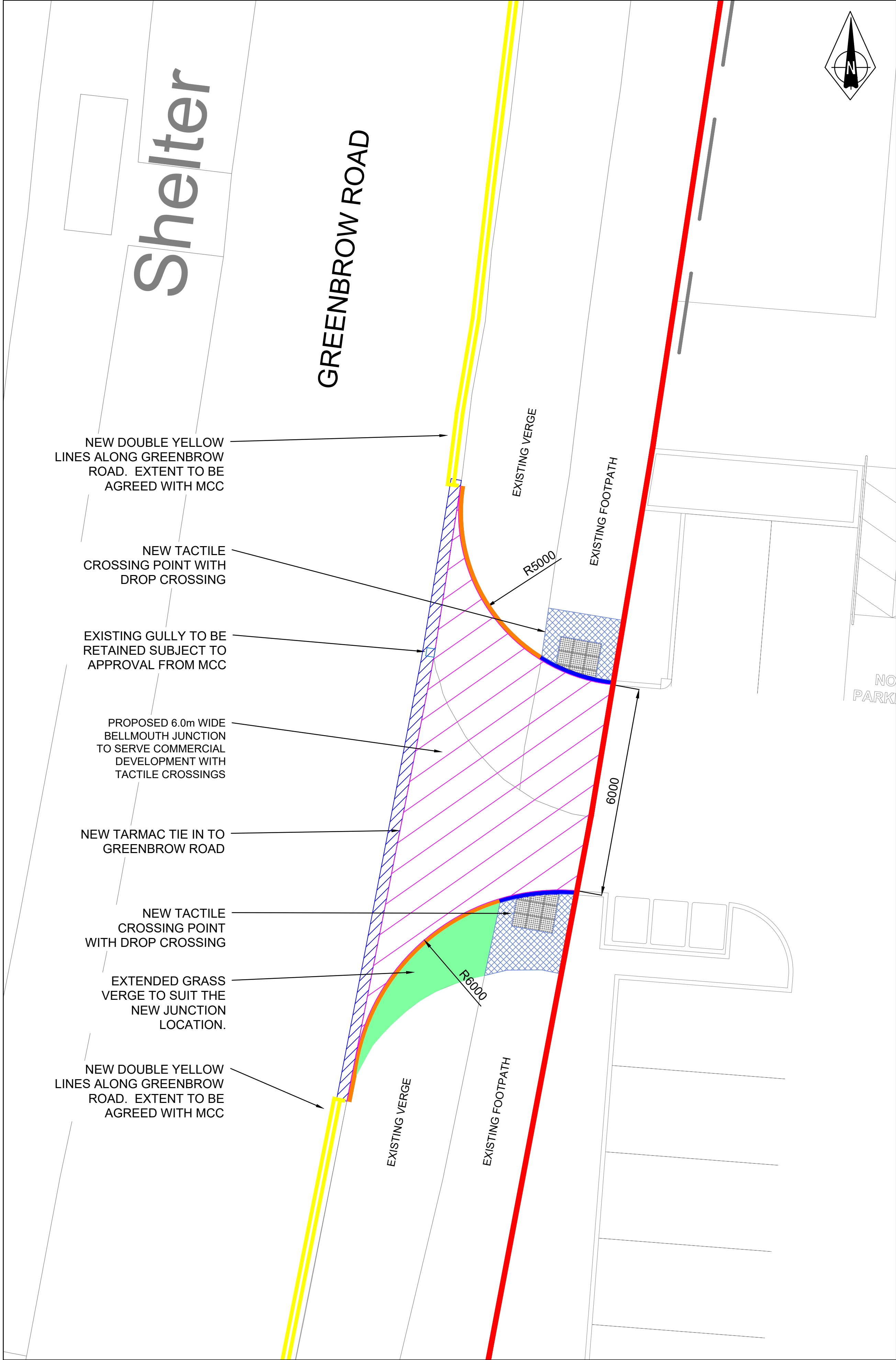
PROPOSED JUNCTION GA
