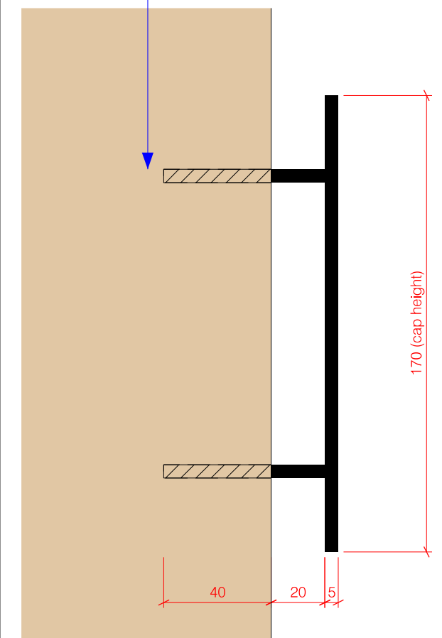
Detail - Fixing 1:2
