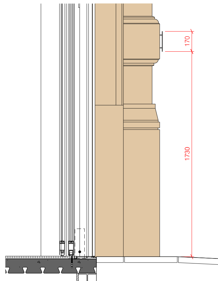
Proposed Section - Setting Out 1:20
