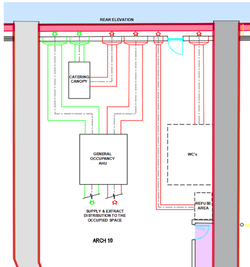
TYPICAL TENANT VENTILATION LAYOUT & TERMINALS FOR ARCH 10 (REAR ELEVATION)
