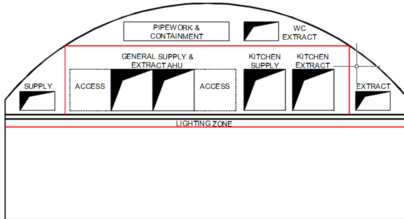
TYPICAL VENTILATION DISTRIBUTION SECTION
