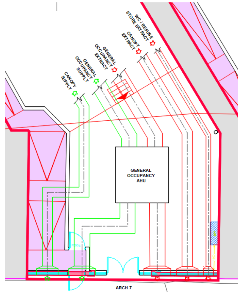
TYPICAL TENANT VENTILATION LAYOUT & TERMINALS FOR ARCH 7 (FRONT ELEVATION)
