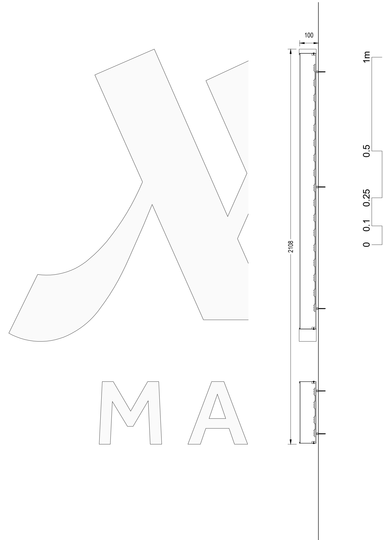
SIGN 5(E) SECTION 1:10
