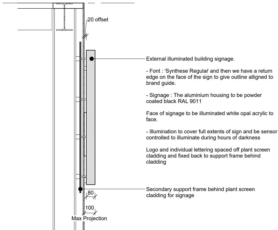
External Signage (High Level) Section
