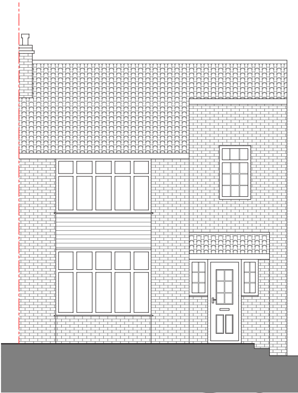
EXISTING FRONT ELEVATION 1:100 @ A3
