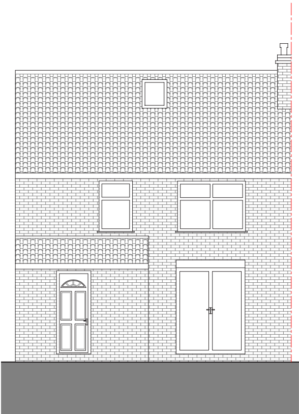
EXISTING REAR ELEVATION 1:100 @ A3
