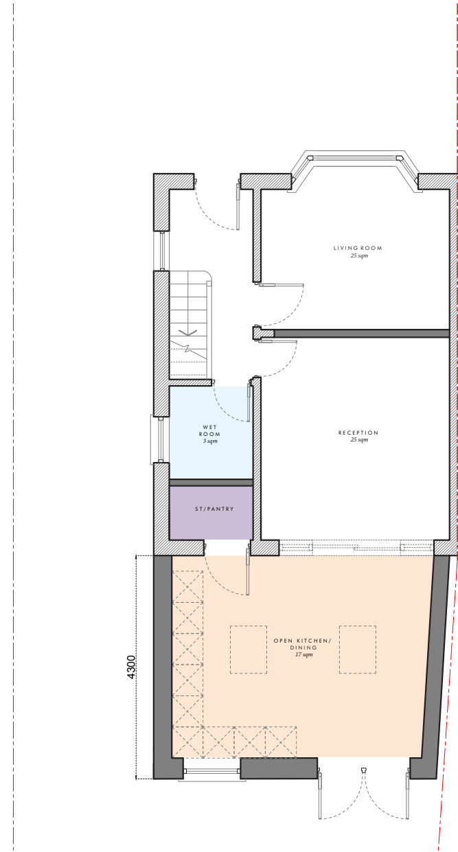
PROPOSED GROUND FLOOR PLAN 1:100 @ A3
