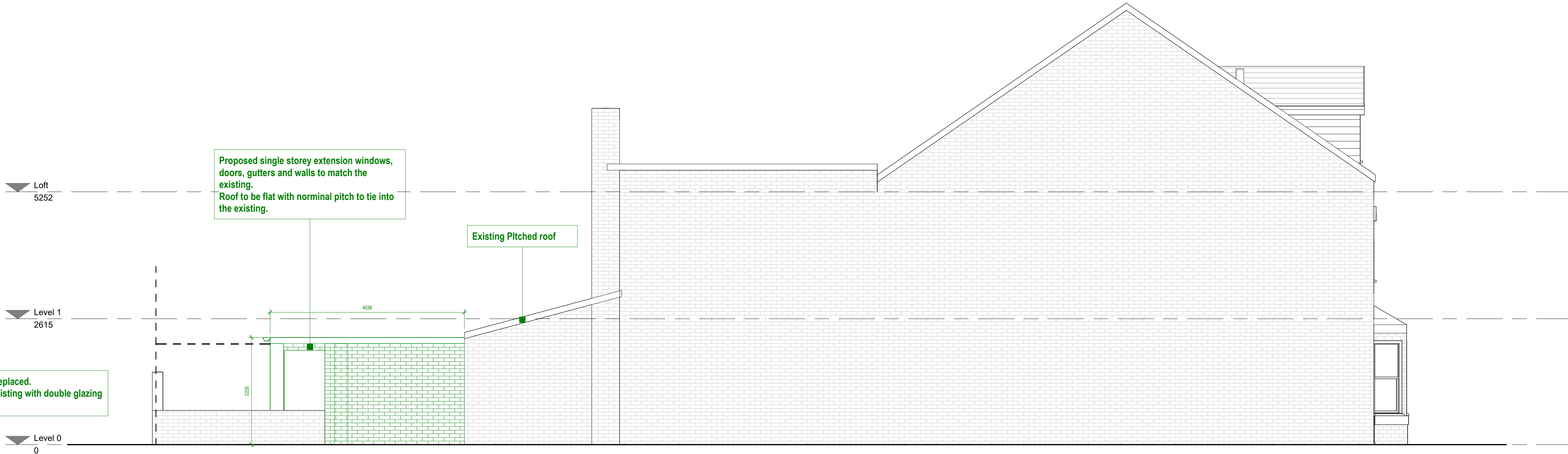
2 Proposed Side 2 Elevation 1:50
