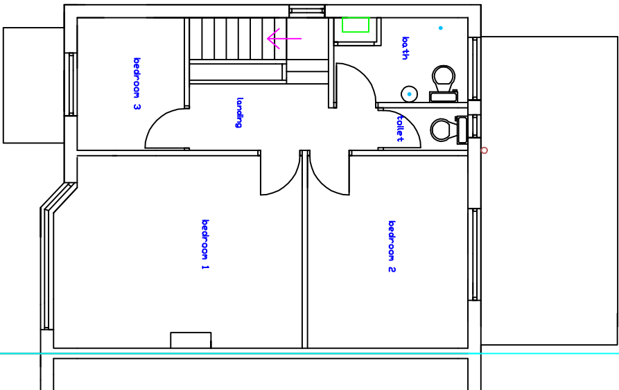
EXISTING FIRST FLOOR 1: 100
