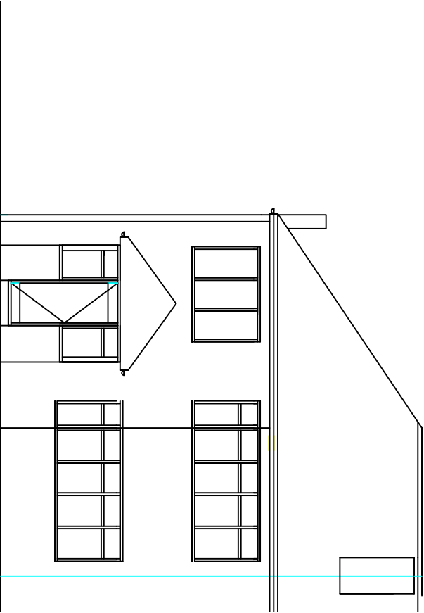
EXISTING FRONT VIEW 1: 100
