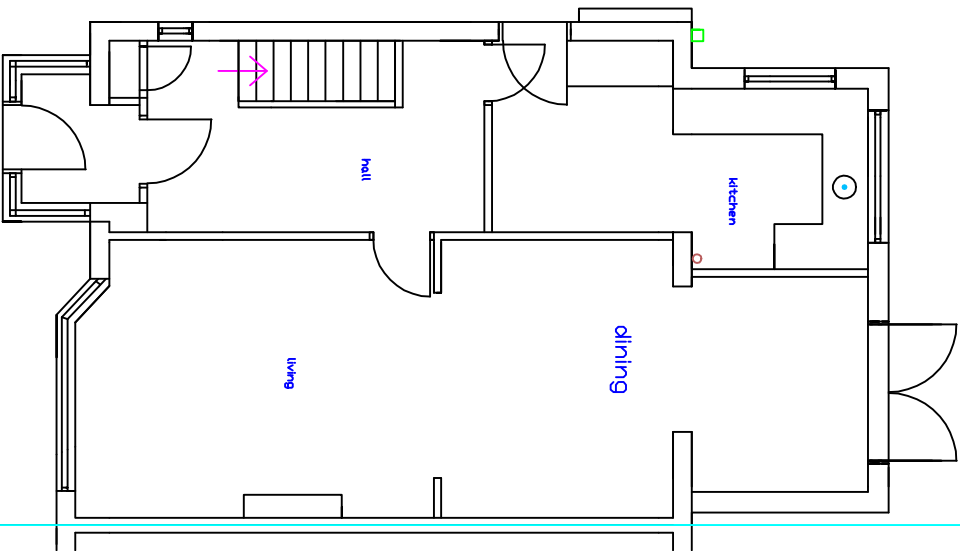
EXISTING GROUND FLOOR 1: 100
