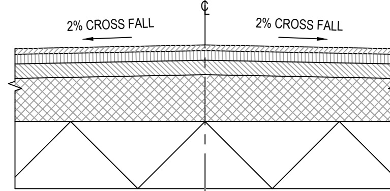
TYPICAL SECTION THROUGH ACCESS ROAD [SCALE: 1:20]
