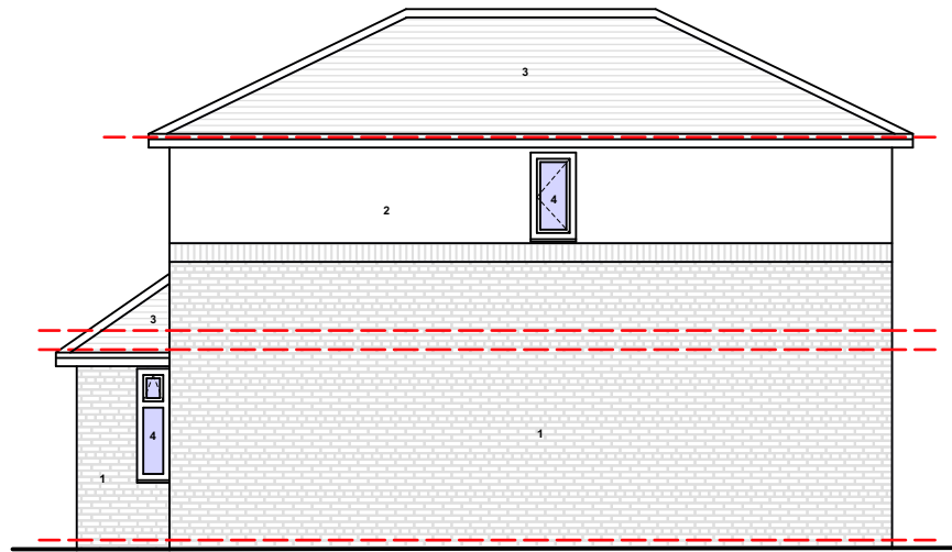
EXISTING GA SIDE ELEVATION 1
