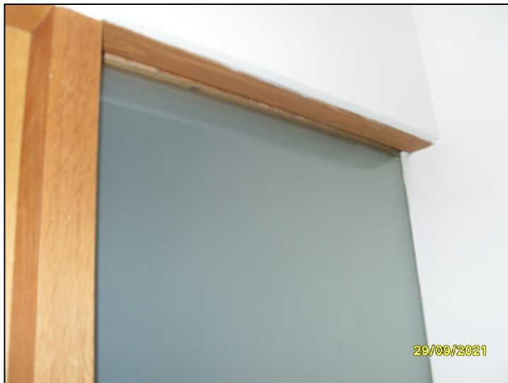
PHOTO 08 – Internal, poorly installed fire rated glazing unit
