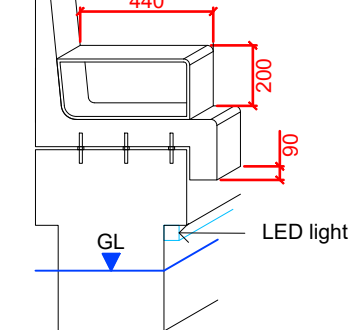
ARM REST DETAIL 014 ISO @ 1:25
