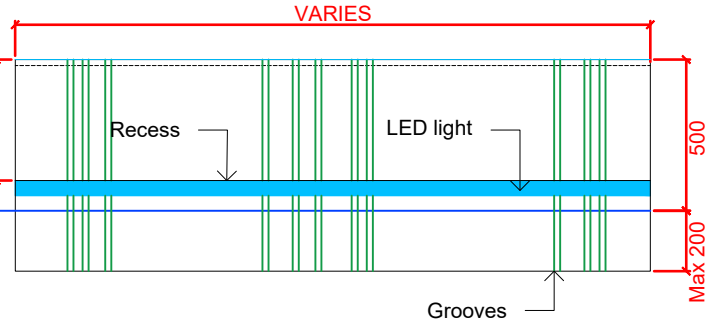
GRANITE BENCH TYPICAL INTERMEDIATE UNIT DETAIL 004 ELEVATION @ 1:25
