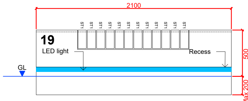
UNIT 19 INC TIMBER TOP DETAIL 013 ELEVATION @ 1:25
