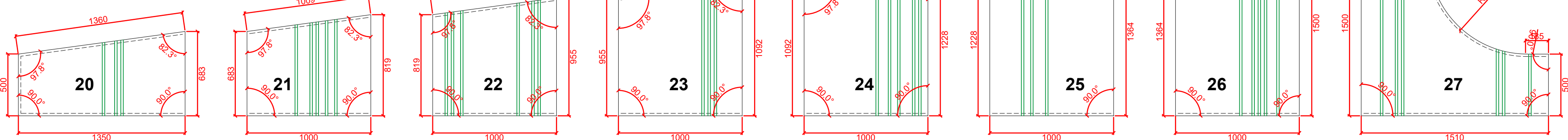
SPECIAL UNITS 20 - 27 DETAIL 015 PLAN @ 1:25
