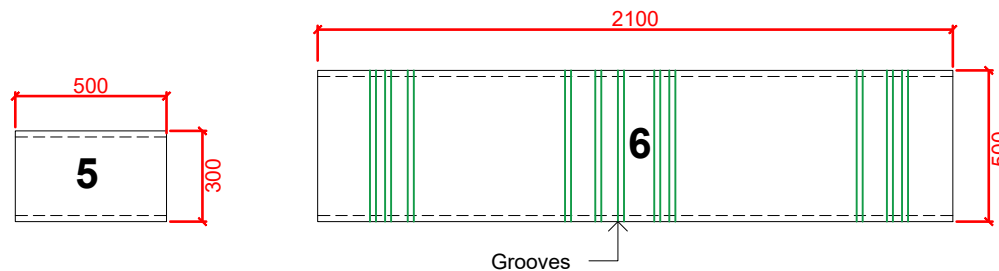
GRANITE BENCH INTERMEDIATE UNITS 5 - 6 DETAIL 002 PLAN @ 1:25
