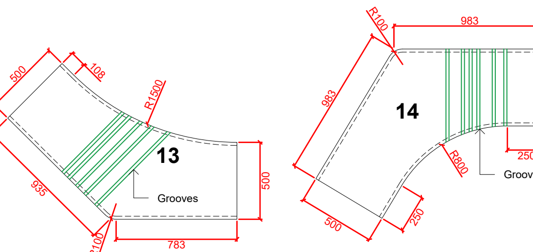
GRANITE BENCH DIRECTIONAL UNITS 13 - 17 DETAIL 007 PLAN @ 1:25
