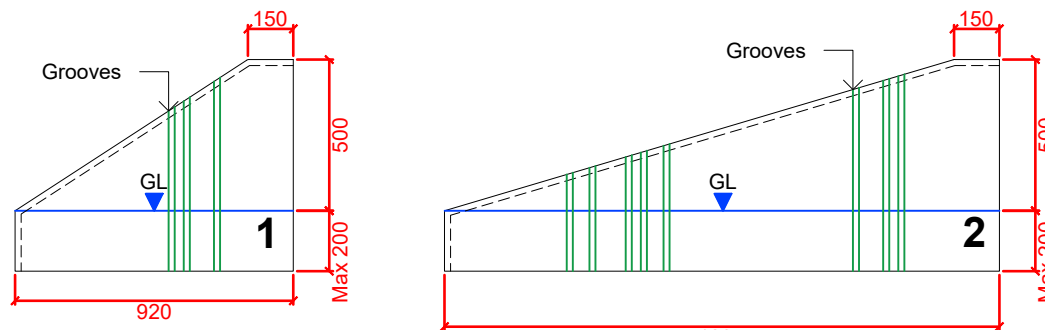
GRANITE BENCH END UNITS 1 - 4 DETAIL 003 ELEVATION @ 1:25
