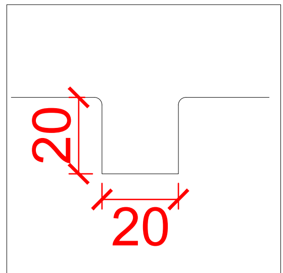
GROOVE DETAIL 016 SECTION @ 1:1
