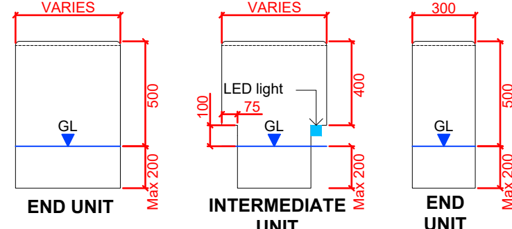
GRANITE BENCH TYPICAL INTERMEDIATE UNIT DETAIL 005 SECTION @ 1:25
