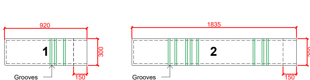
GRANITE BENCH END UNITS 1 - 4 DETAIL 001 PLAN @ 1:25
