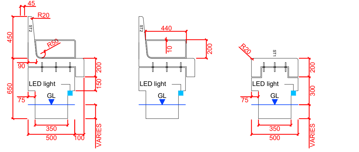
UNIT 18 INC TIMBER TOP ARM & BACK REST DETAIL 008 SECTION @ 1:25
