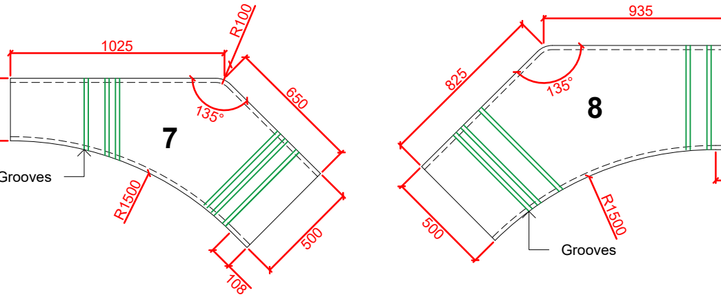
GRANITE BENCH DIRECTIONAL UNITS 7 - 12 DETAIL 006 PLAN @ 1:25
