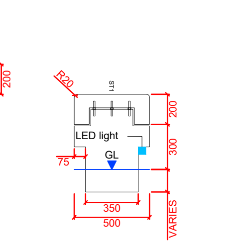
UNIT 19 INC TIMBER TOP DETAIL 009 SECTION @ 1:25
