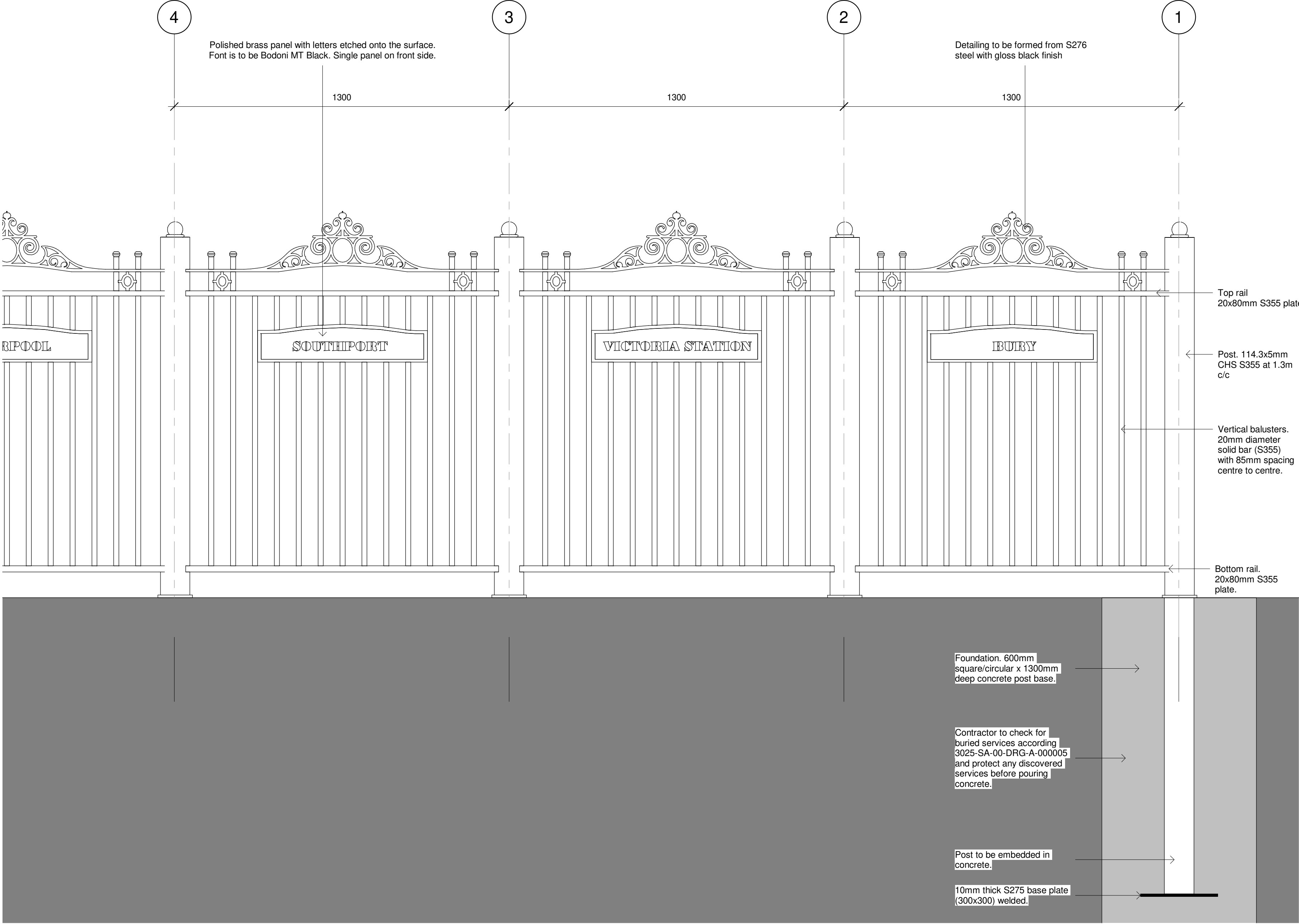
1 Proposed Elevation Detail 1 : 10
